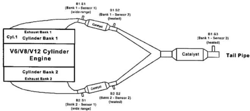
V6/V8/V12 Engine W/2 Exhaust Banks & 3 Catalyts
