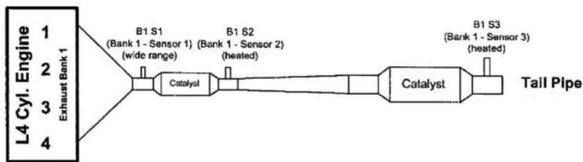
L4 Engine W/1 Exhaust Banks & 2 Catalyts
