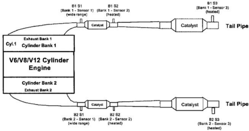
V6/V8/V12 Engine W/2 Exhaust Banks & 4 Catalyts
