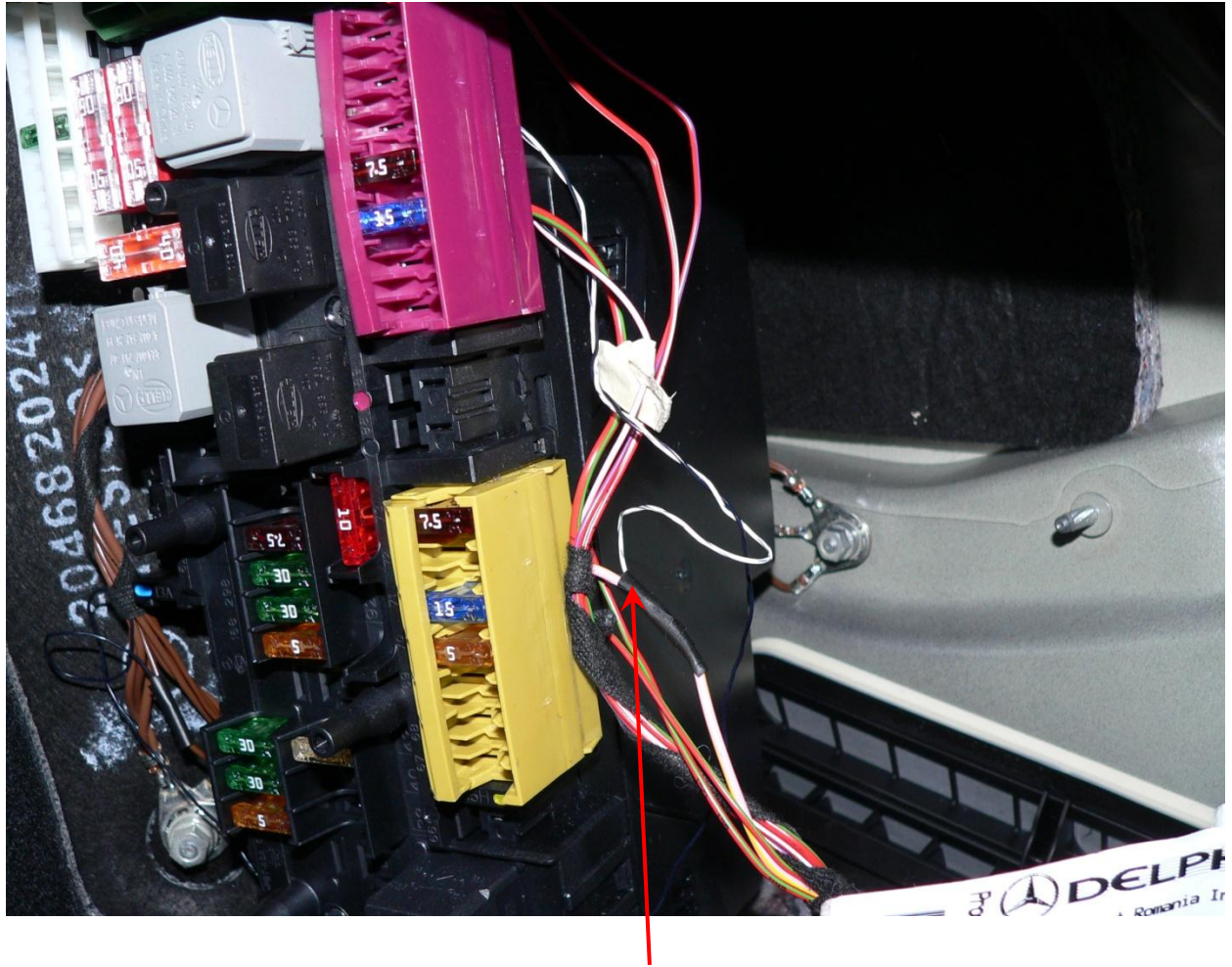
Red arrow points at fuse # 71 wire. Wire color is like very light brown. The other thin wire just above the red arrow is the camera power wire, soldered and taped onto fuse wire.
