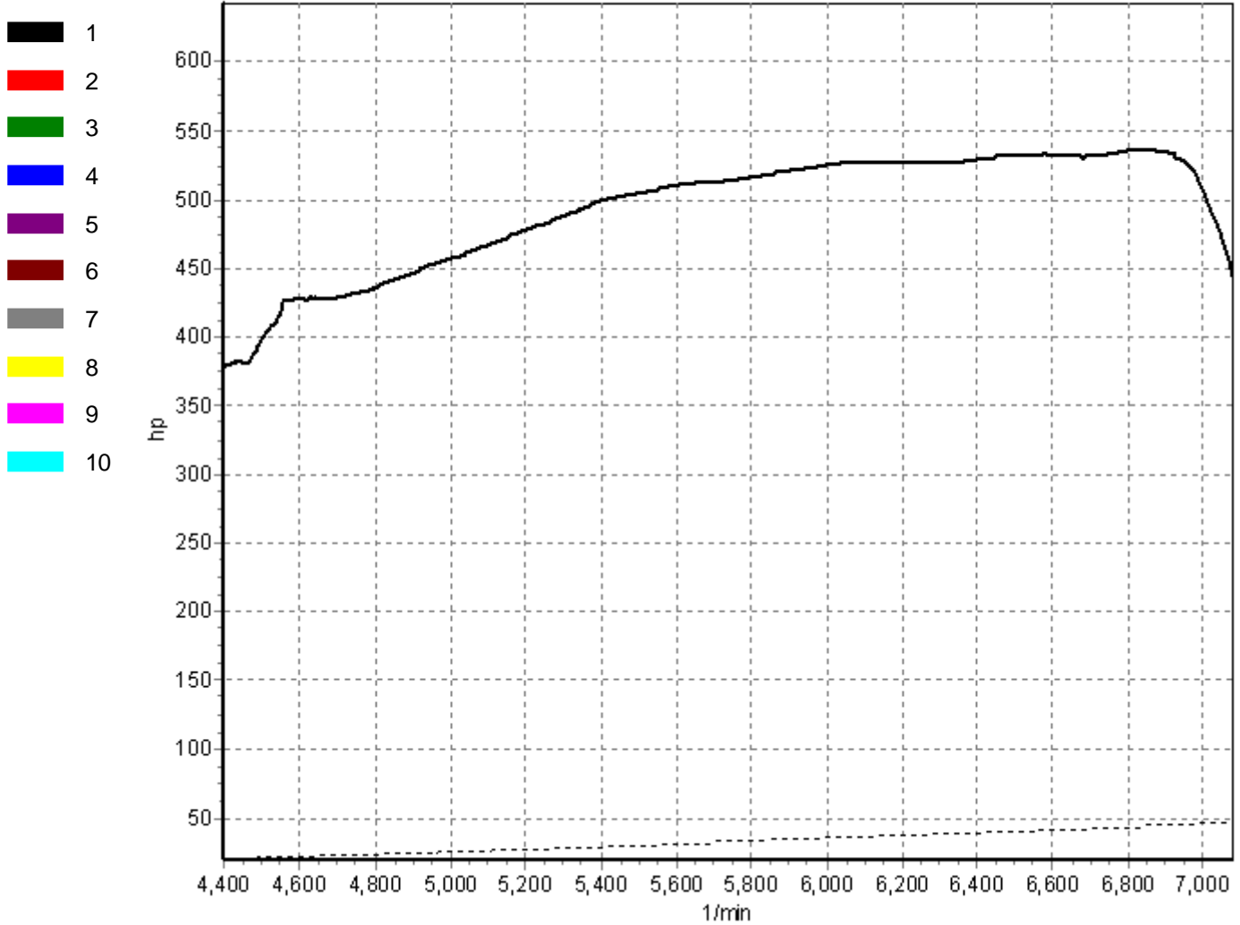
P-max Engine power (meas.) / Power Losses (gem.) / Speed
