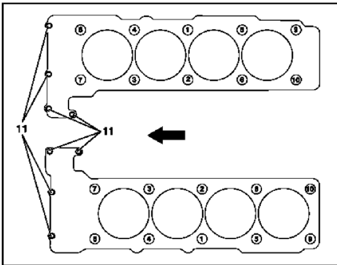
Tightening scheme Schematic diagram of cylinder head gasket
