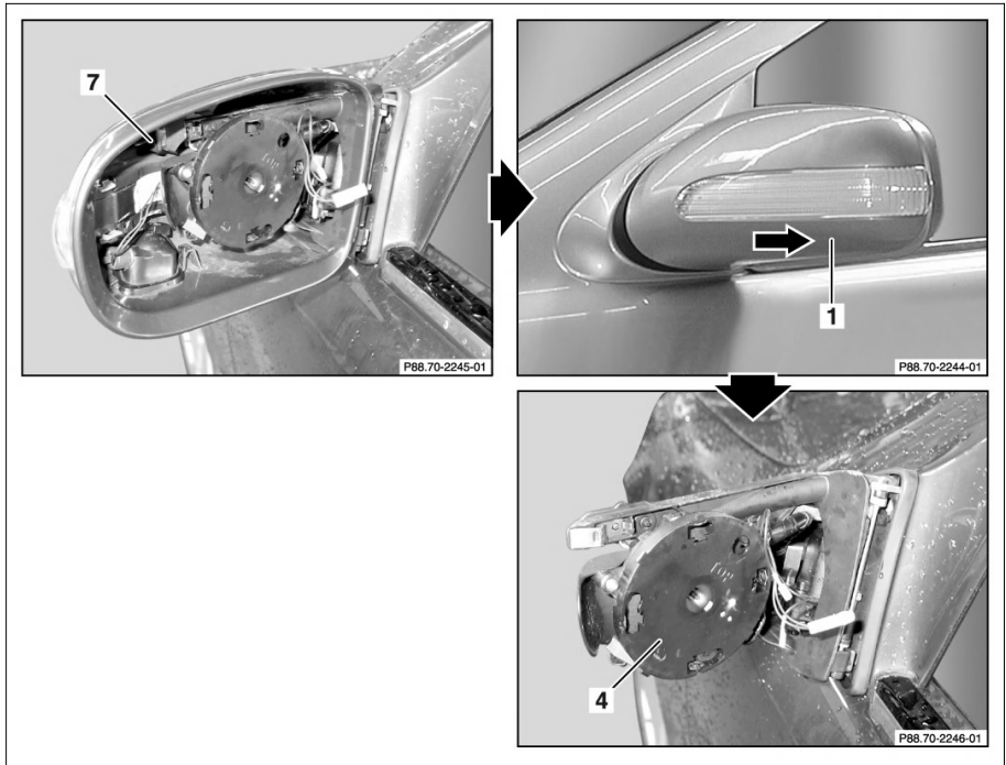
P88.70-2243-06
