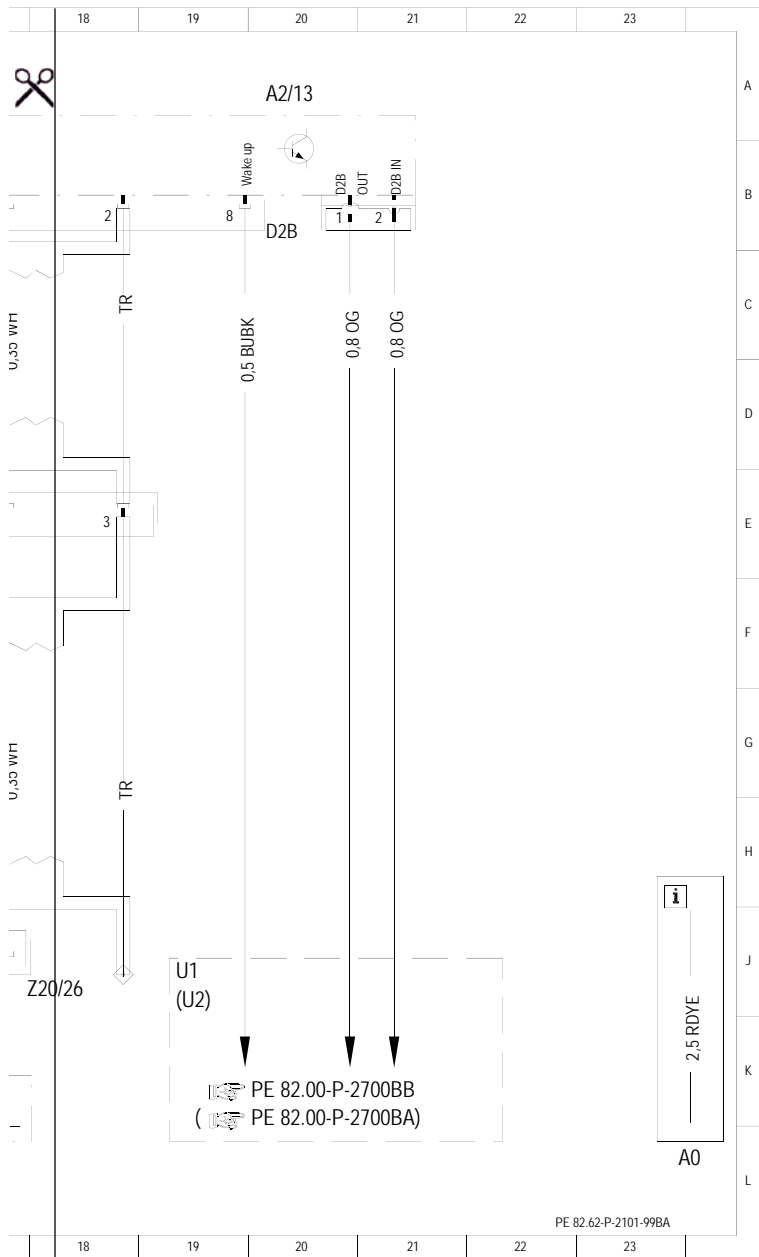
Sound amplifier control unit wiring diagram / pe82.62-p-2101-99ba MODEL 209 control unit A2/13 with D2 bus / Printed on: 21.11.2013 / Page 2/2
