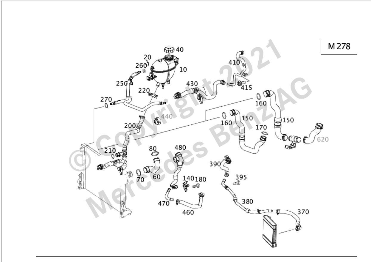
Image ID: drawing_B50165000416
