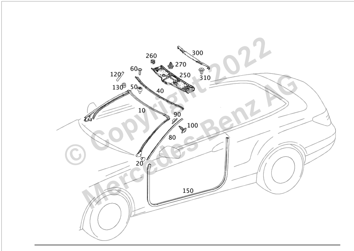
Image ID: drawing_B69015000300
