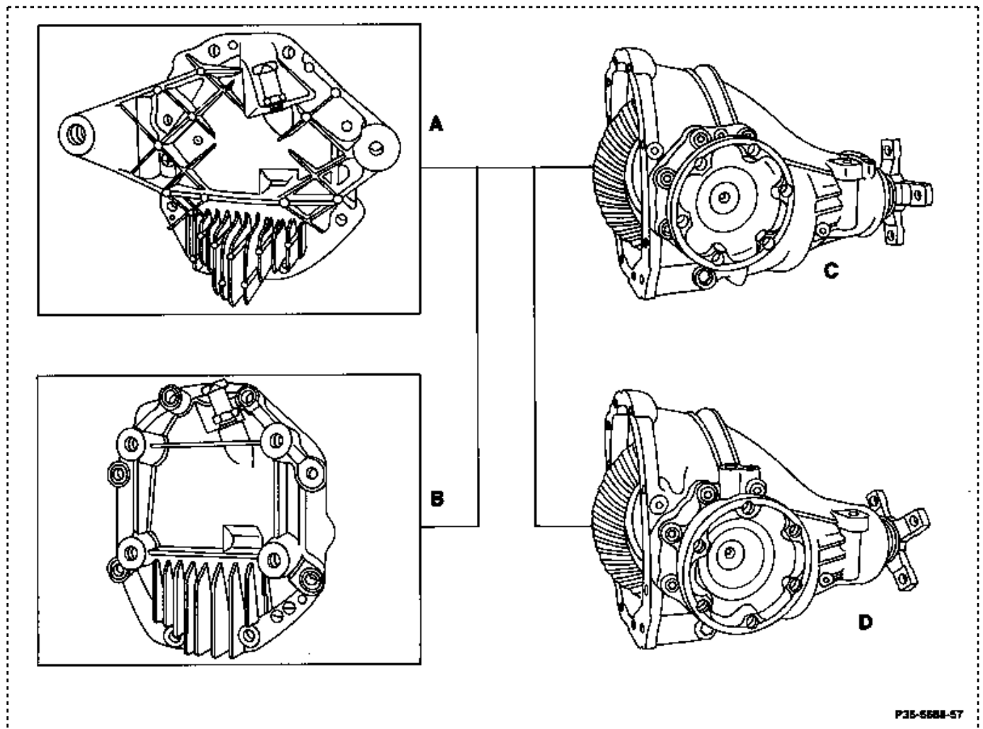
A Rear axle end cover, model 129 B Rear axle end cover, model 140
