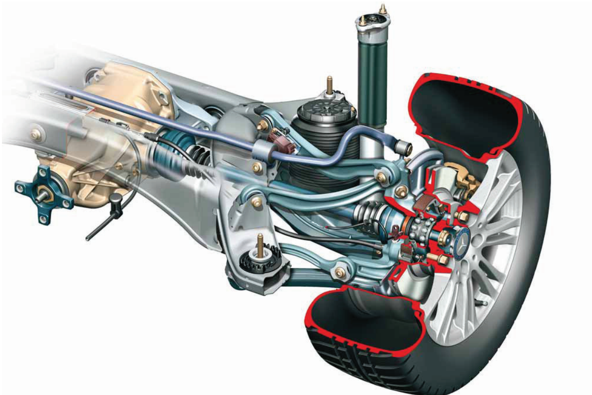
Rear axle with AIRMATIC air suspension (E 550)
