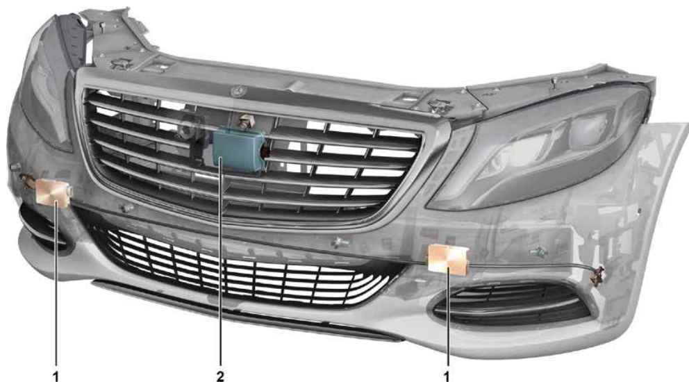
Installation situation of DTR+ radar sensors (code 233)
