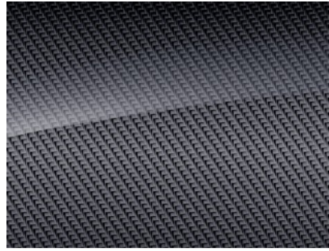
H62 - Carbon Structure
