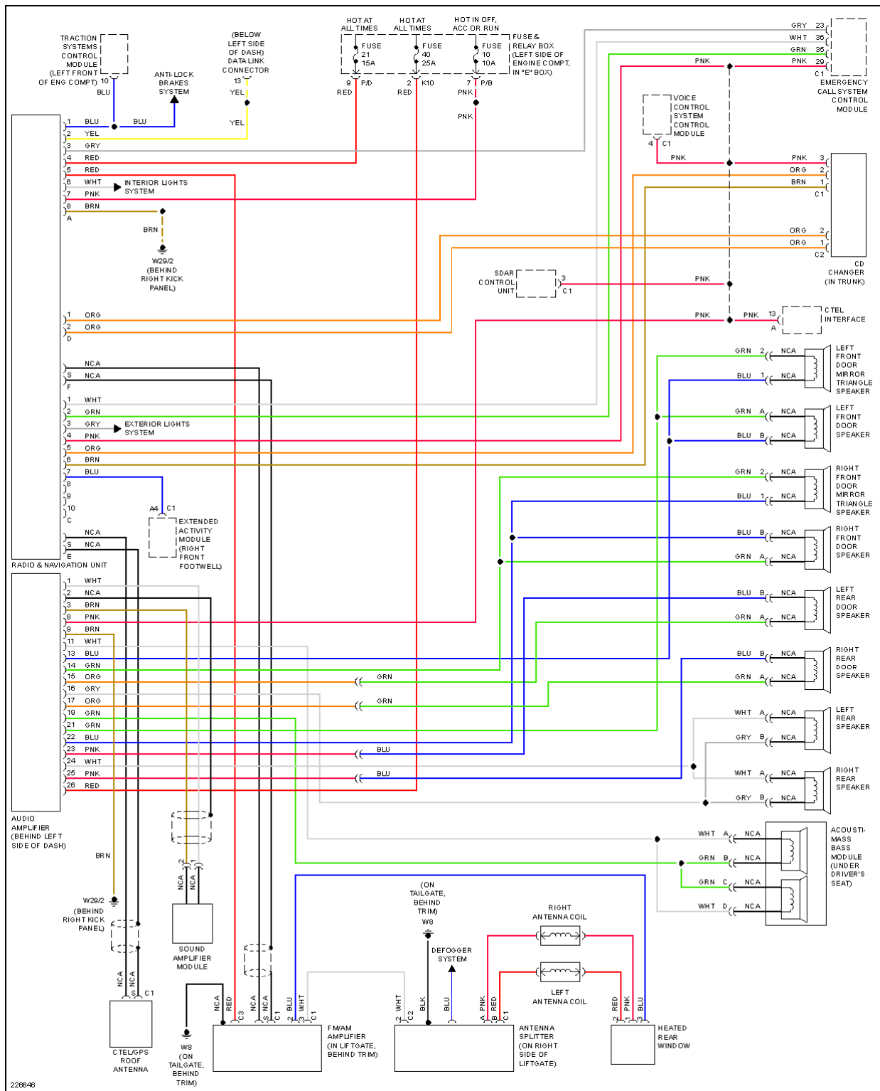
Fig. 50: Bose Radio Circuit
