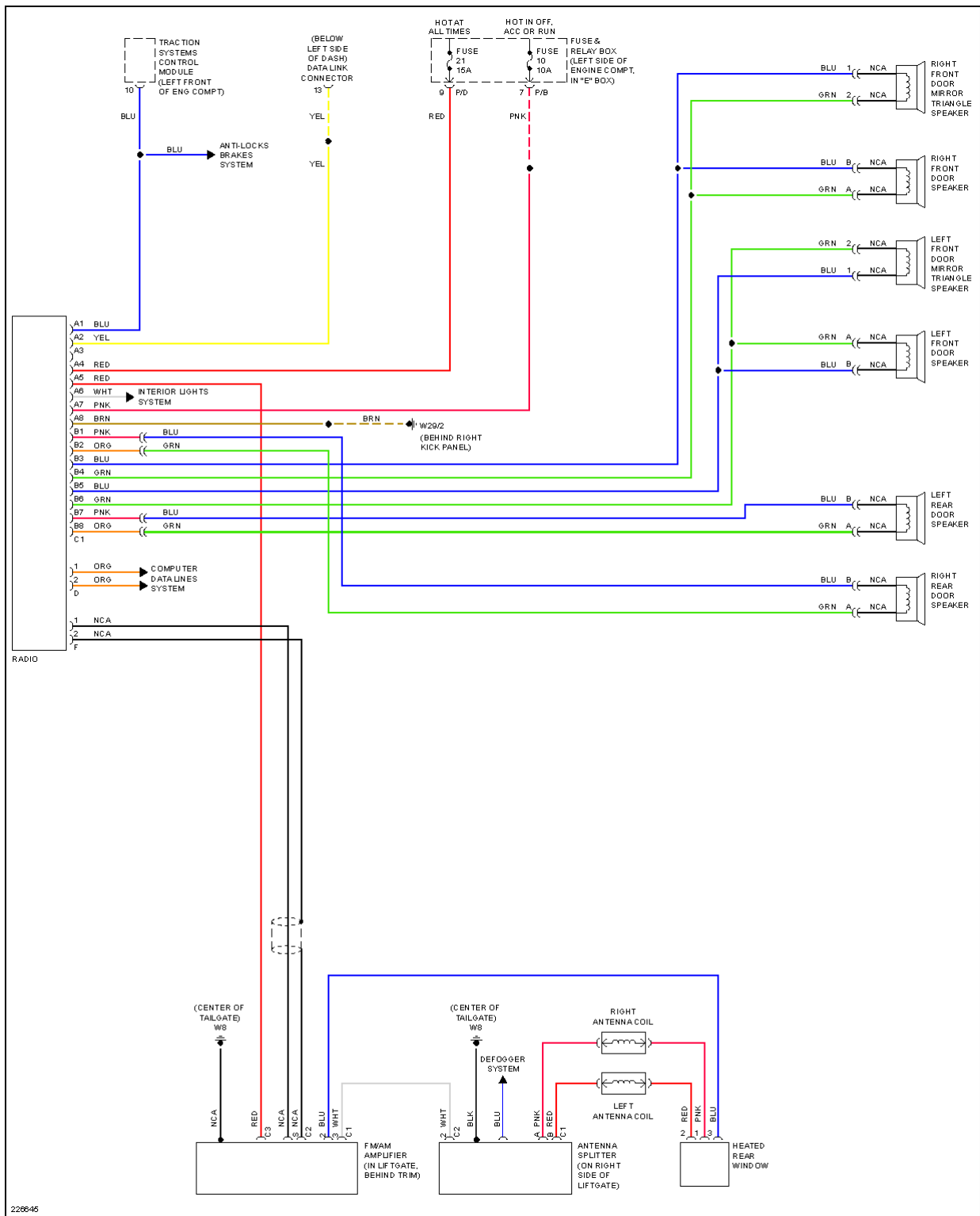
Fig. 49: Base Radio Circuit
