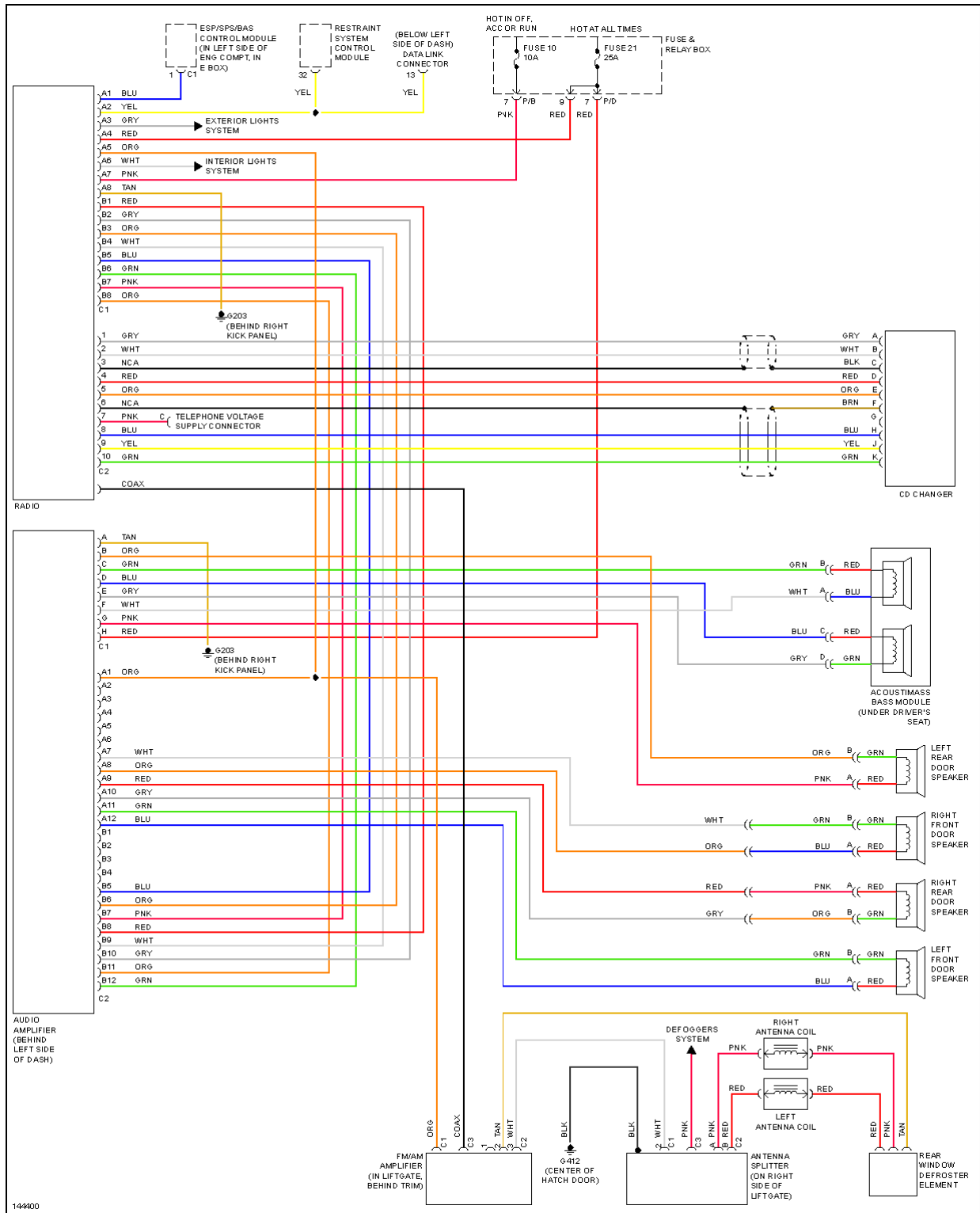
Fig. 50: Radio Circuits, Premium Radio
