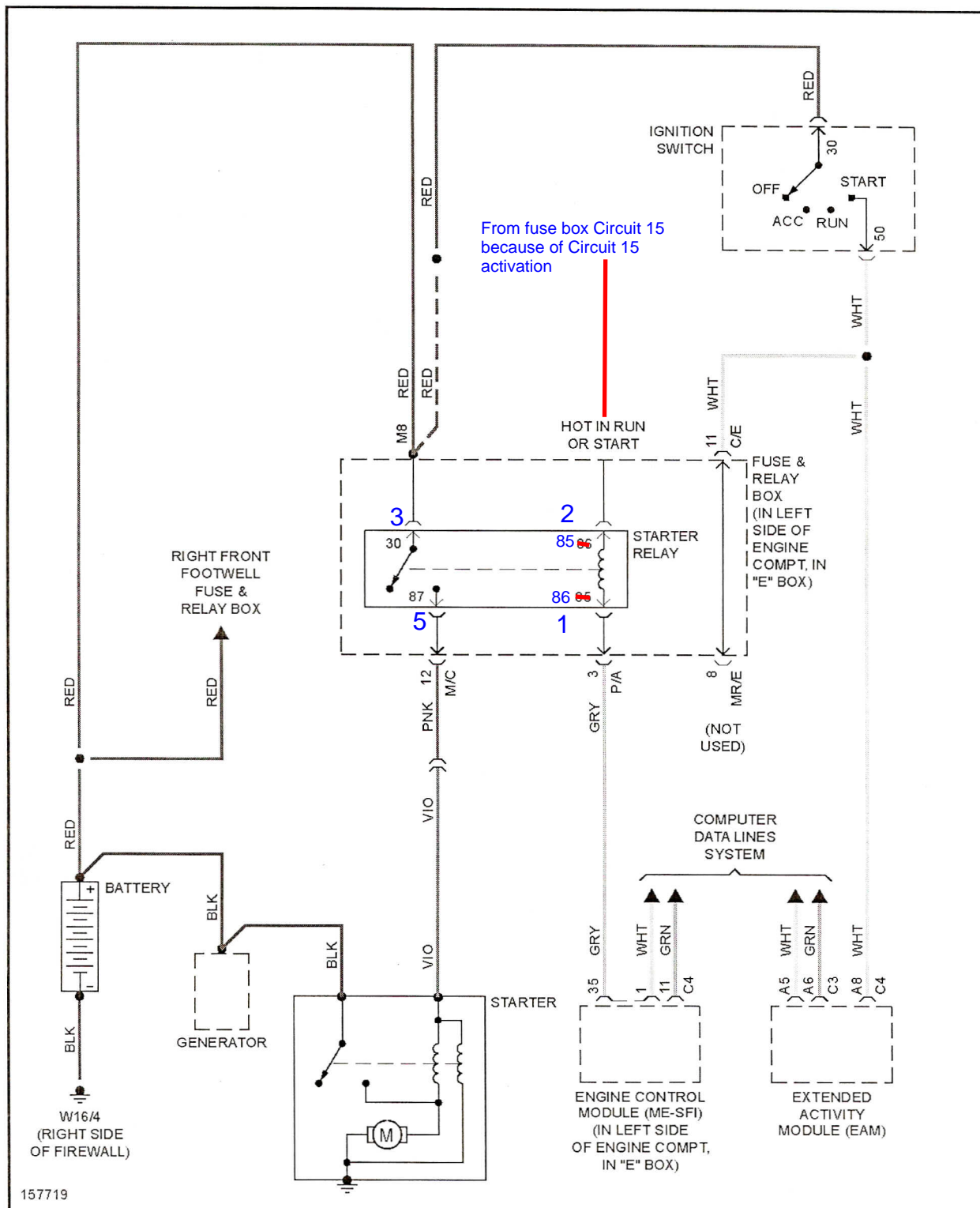
Fig. 54: Starting Circuit
