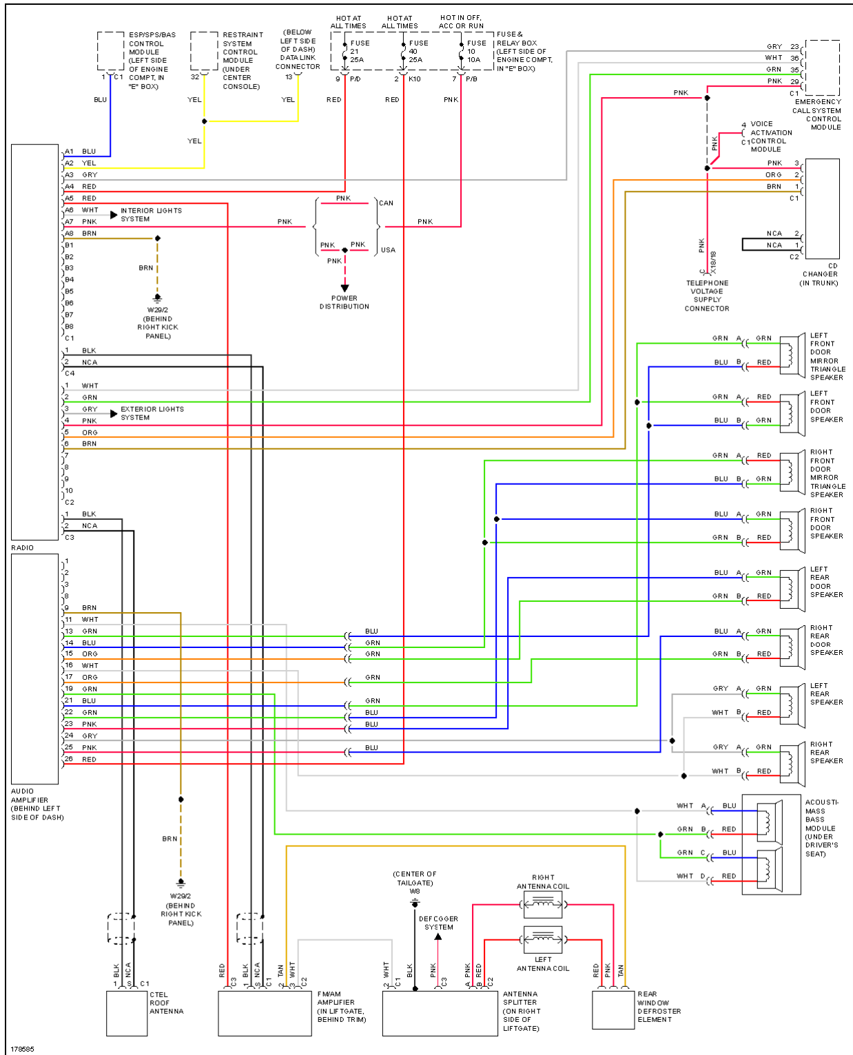
Fig. 50: Radio Circuit, Bose
