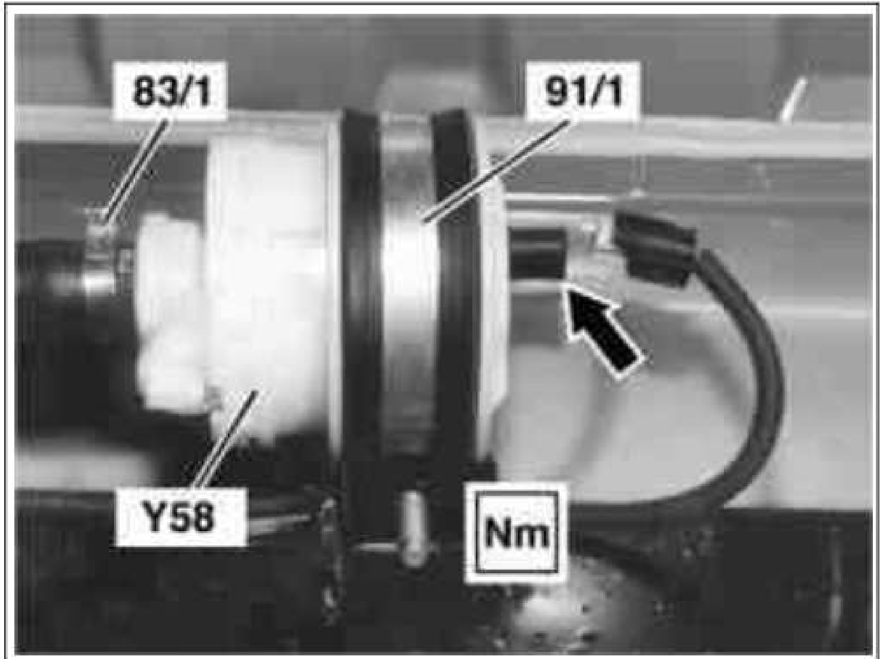
As of 2001 this valve was moved to the right rear wheel close to the fuel tank.
