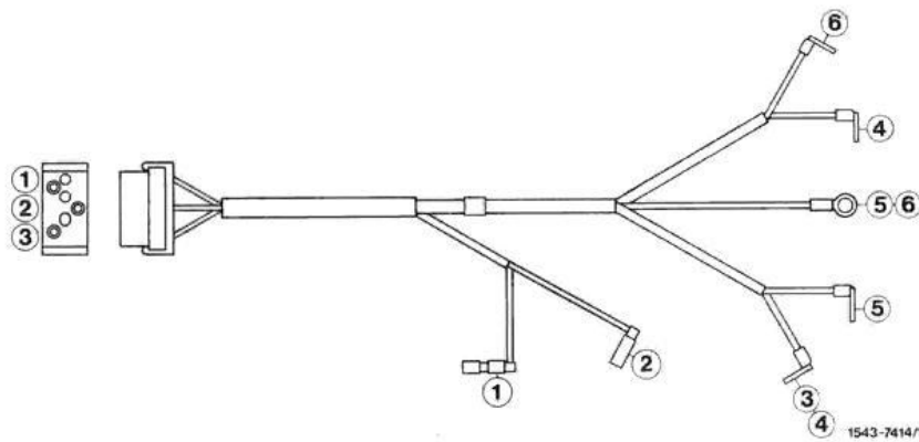
Color code of supplementary harness
