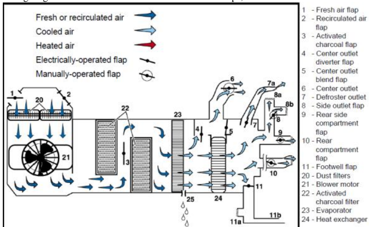
Figure 1 Definition of W220 Automatic Climate Control (ACC) Flaps/Vents/Outlets
