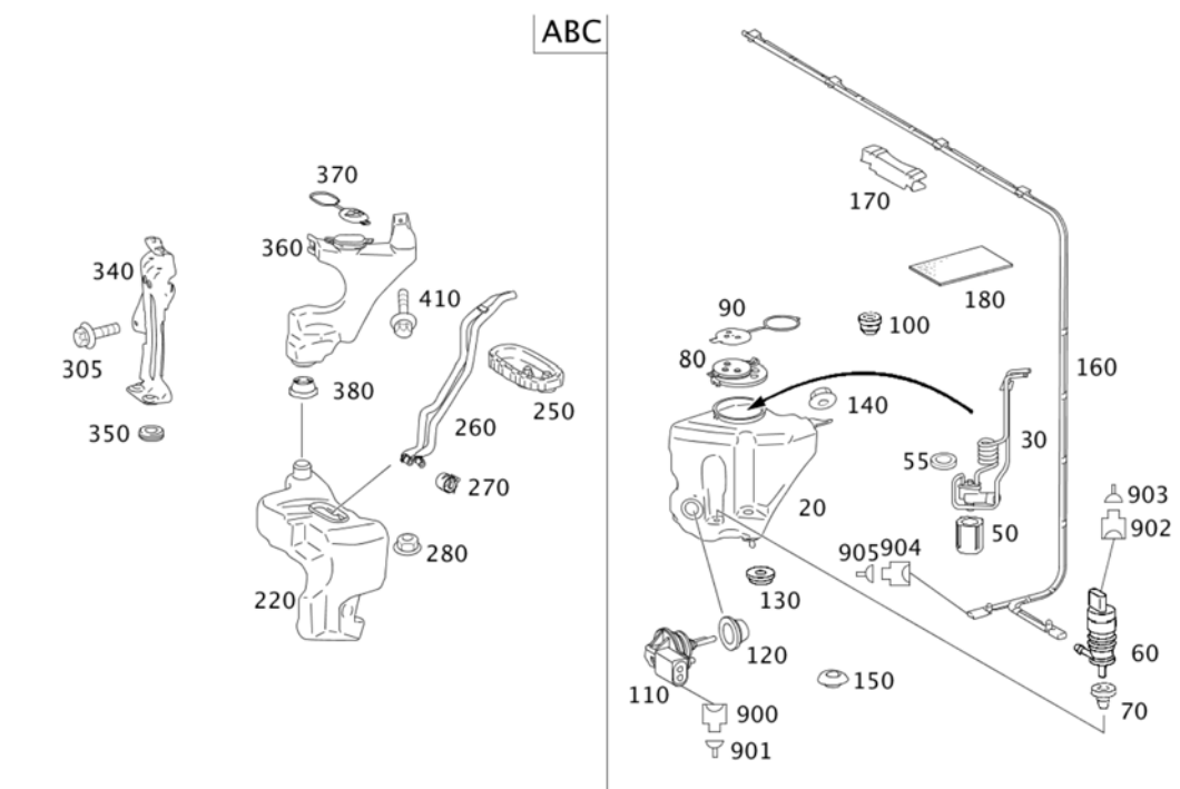
Image ID: drawing_B86030000231
