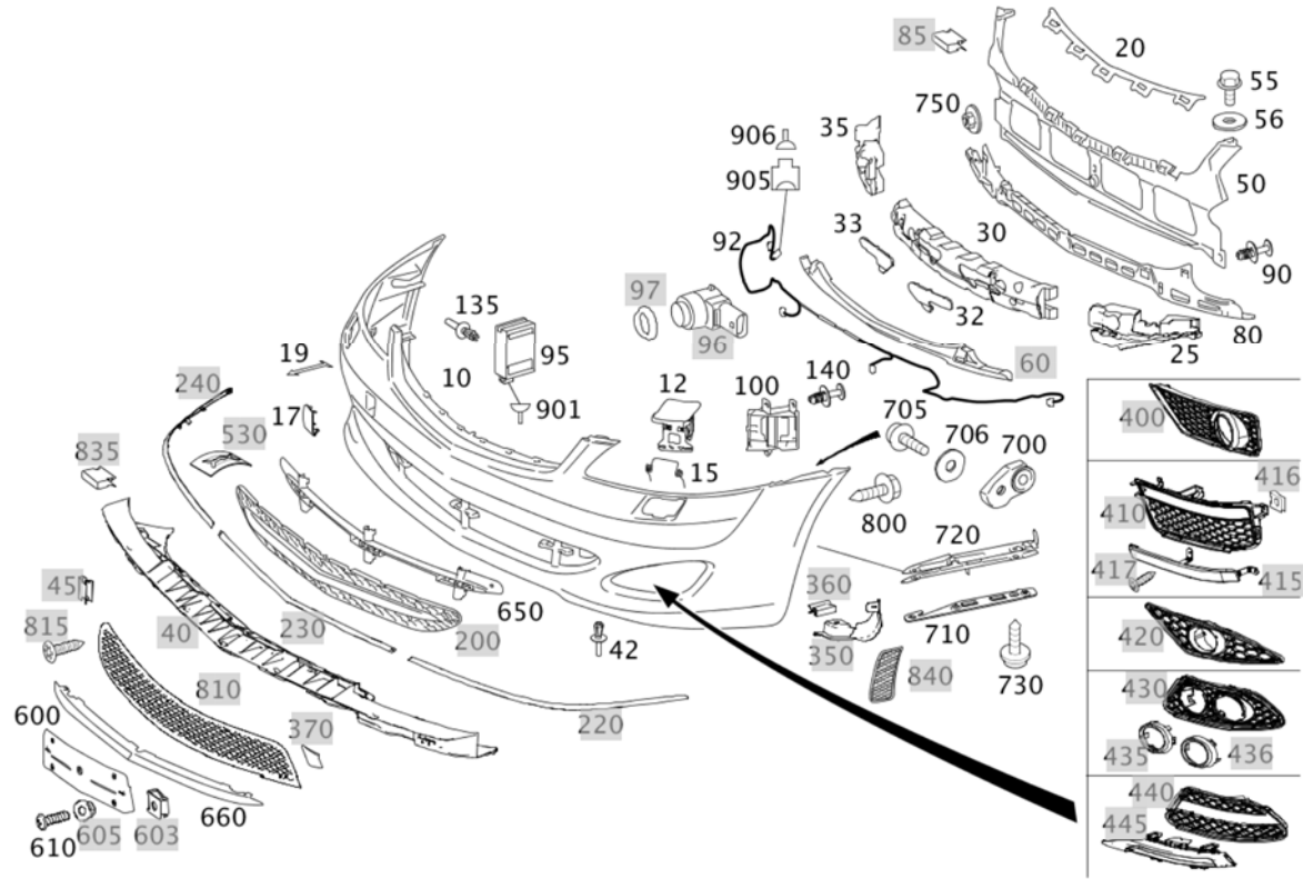
Image ID: drawing_B88030000216
