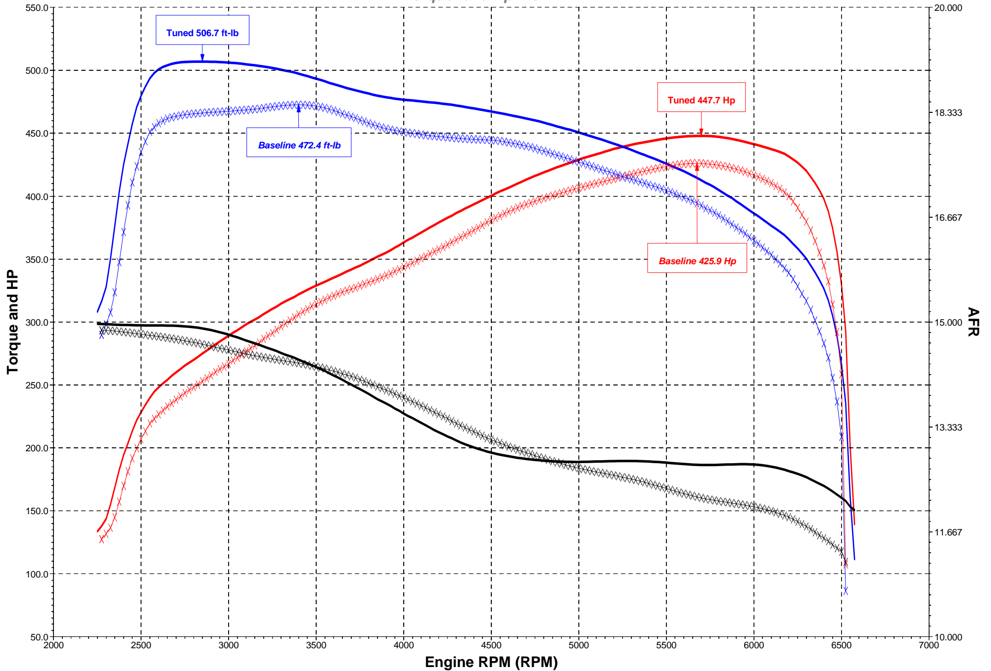
Torque* and Hp* vs. RPM
