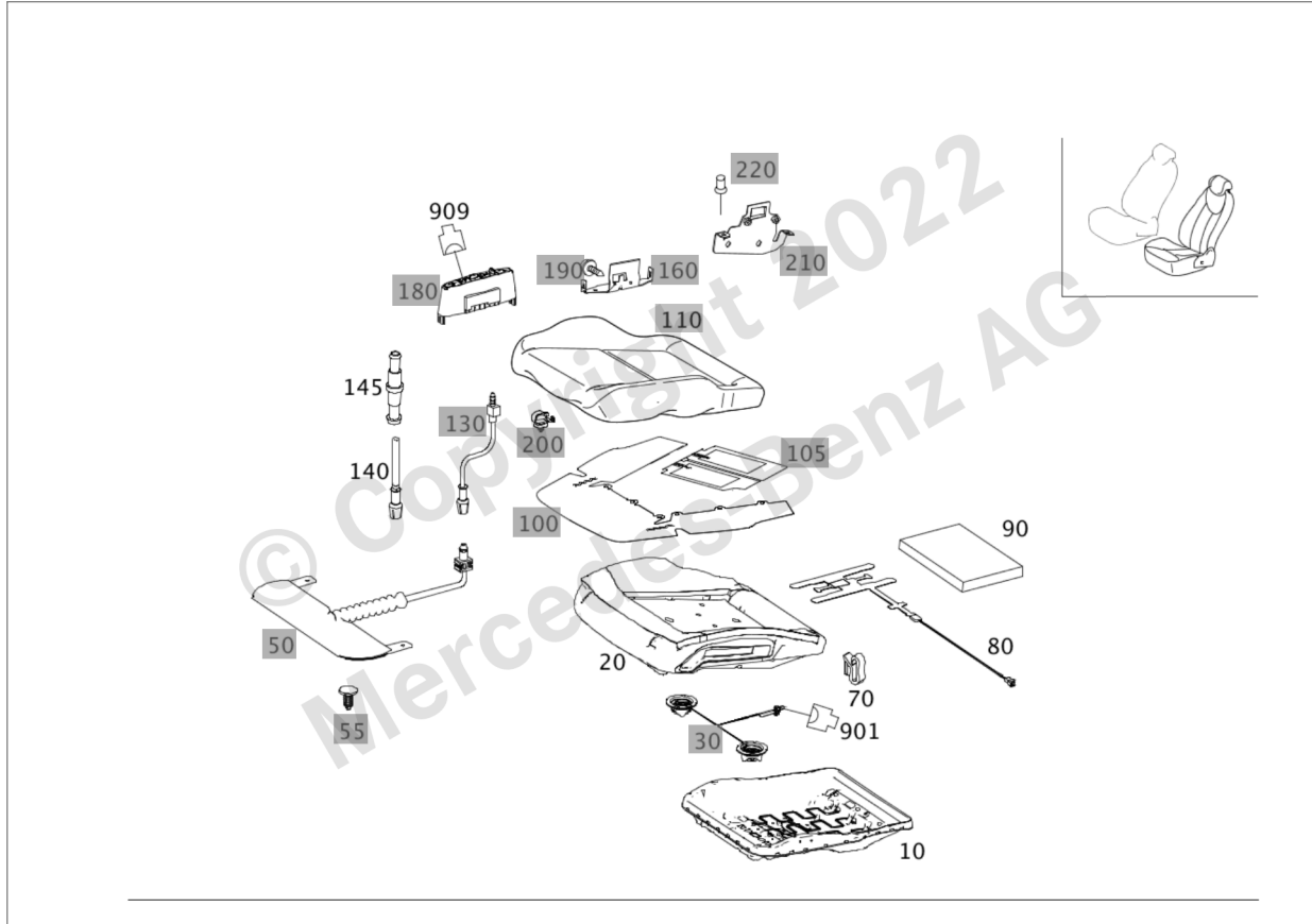
Image ID: drawing_B91065000142
