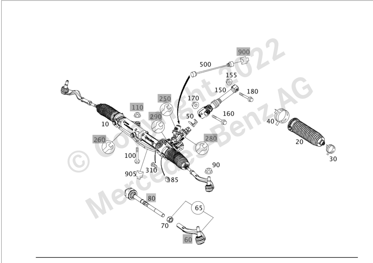
Image ID: drawing_B46015000103
